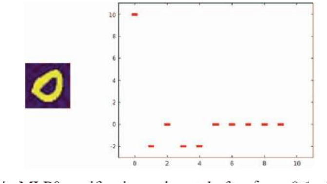
Figure 2: MLP0 verification mismatch for \delta = 0.1 .
