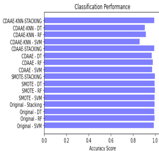
Fig 10: Accuracy Graph
