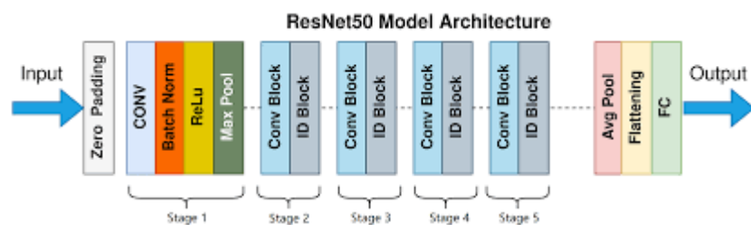
Figure 1: ResNet50 architecture
