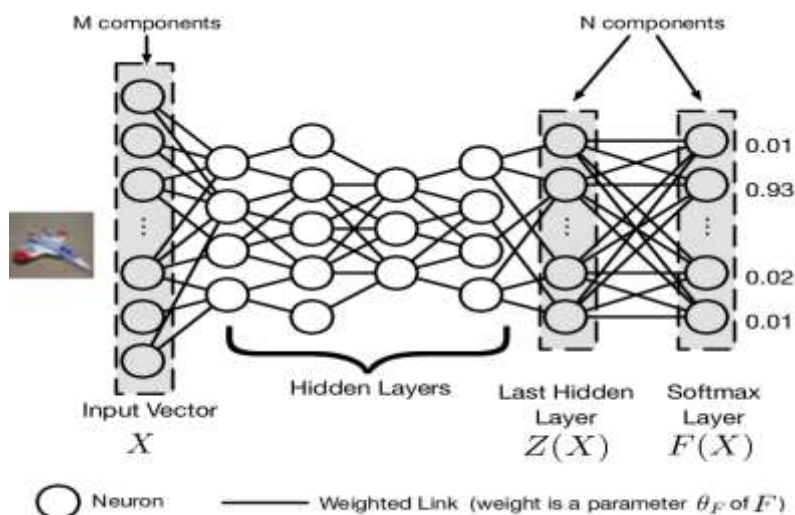
Fig 1: Architecture of DNN
