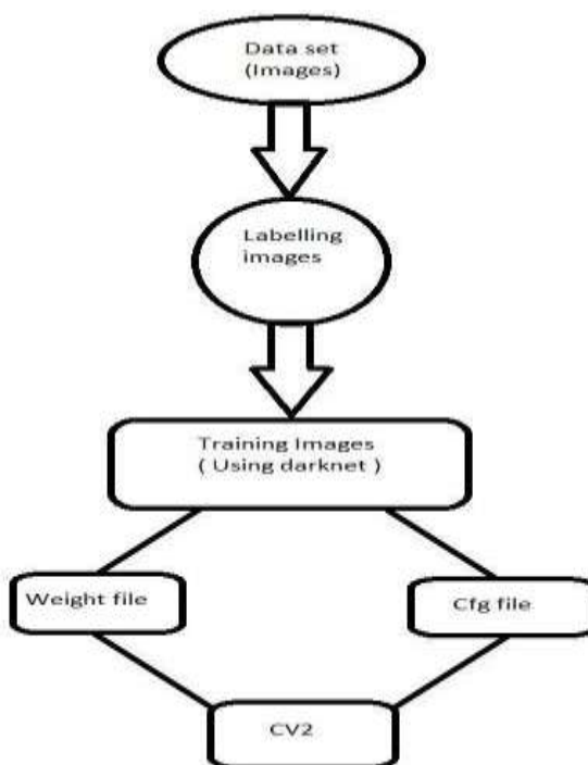
Fig. 1. Data Flowchart
