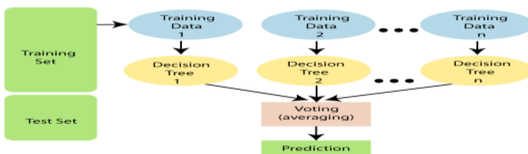
Fig.3. RFA network
