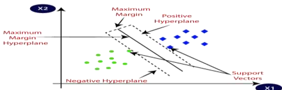
Fig.2. SVM network
