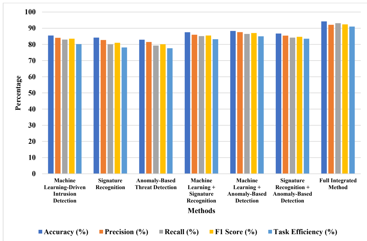
Figure 4 Performance Comparison of Different Cloud Security Approaches Using Machine Learning-Based Detection Systems
