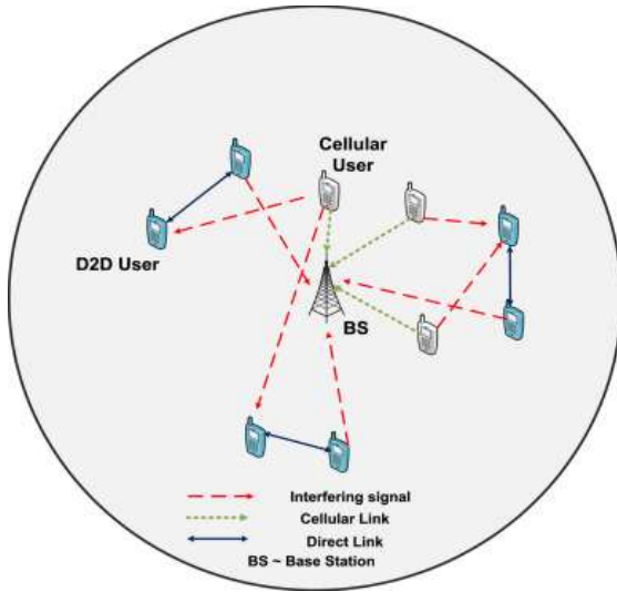
Fig 1 system model of whole cellular network underlaid with D2d communication
