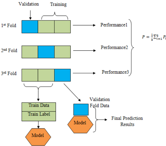
Fig. 7 The concepts of K-Fold cross validation
