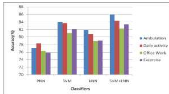
Fig.7: GiST Accuracy graph
