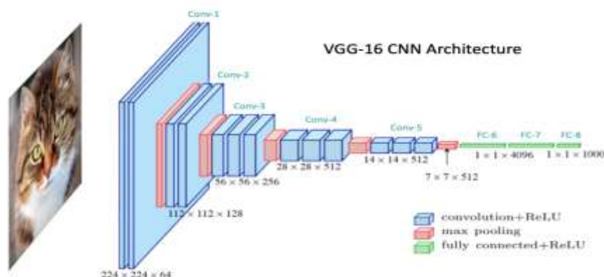
Figure 4.2: Architecture diagram of VGG16 model.
