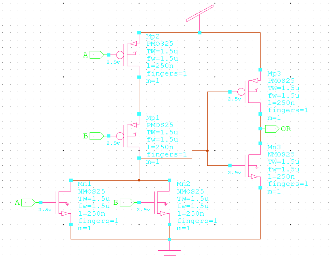
Fig3.5:ORSCHEMATIC
