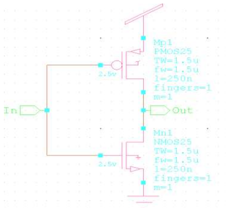
Fig3.2: INVERTER SCHEMATIC
