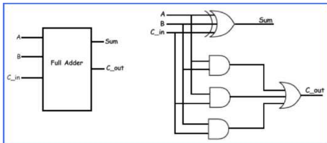
Fig 3.1:One-bitfulladder
