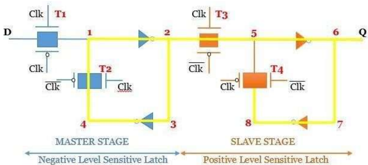
Fig4.2.2: when Clk is high
