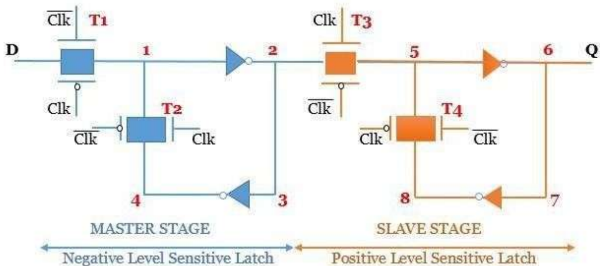
Fig4.1:Positiveedge-triggeredDFFusingTransmissiongate
