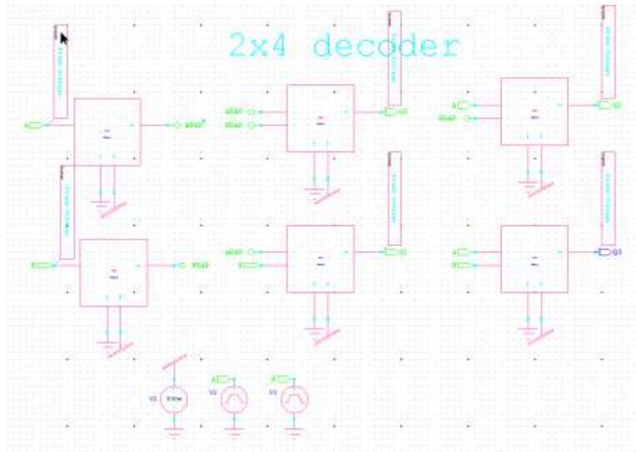
Fig4.1:2*4 Decoder design using16nm technology
