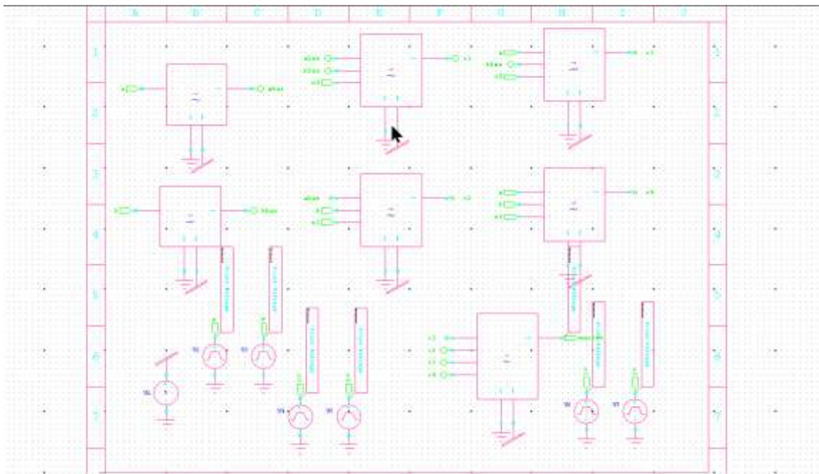
Fig4.1:4*1muxdesignusing16nmtechnology
