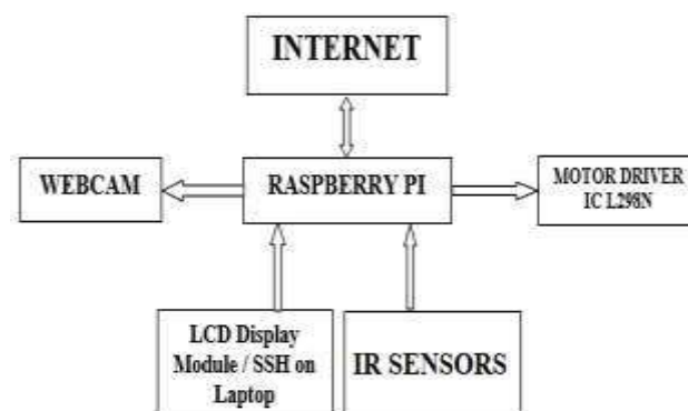
Figure 2: Block Diagram
