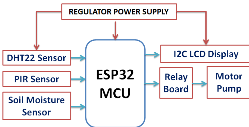
Fig.1: Block Diagram
