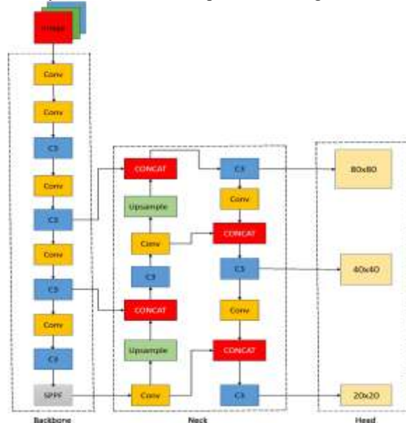
Fig.1. System architecture
