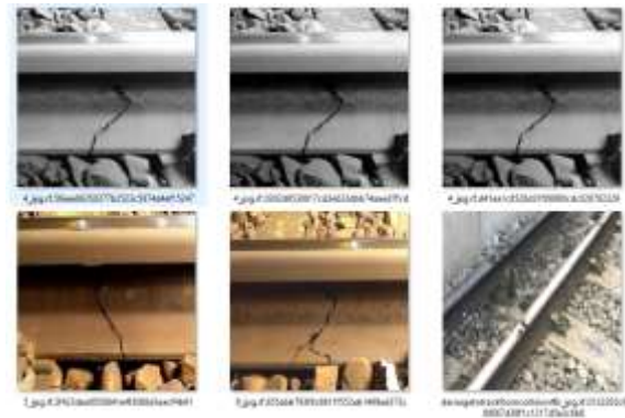
Fig.2. Dataset Collection
