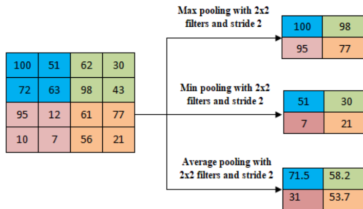
Figure 9 Max, Min and Average Pooling Layer with 2x2 Filters and Stride 2
