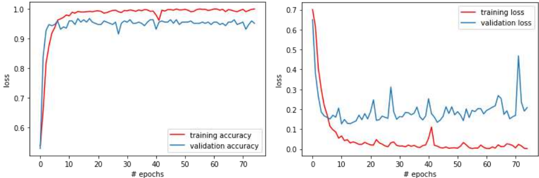
Figure 13 Training and validation accuracy and loss
