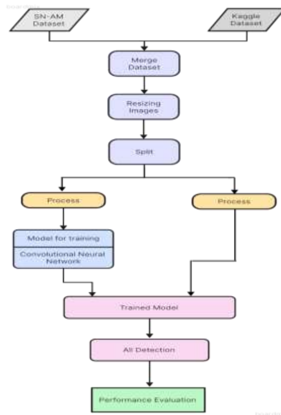
Fig 1: DR methodology
