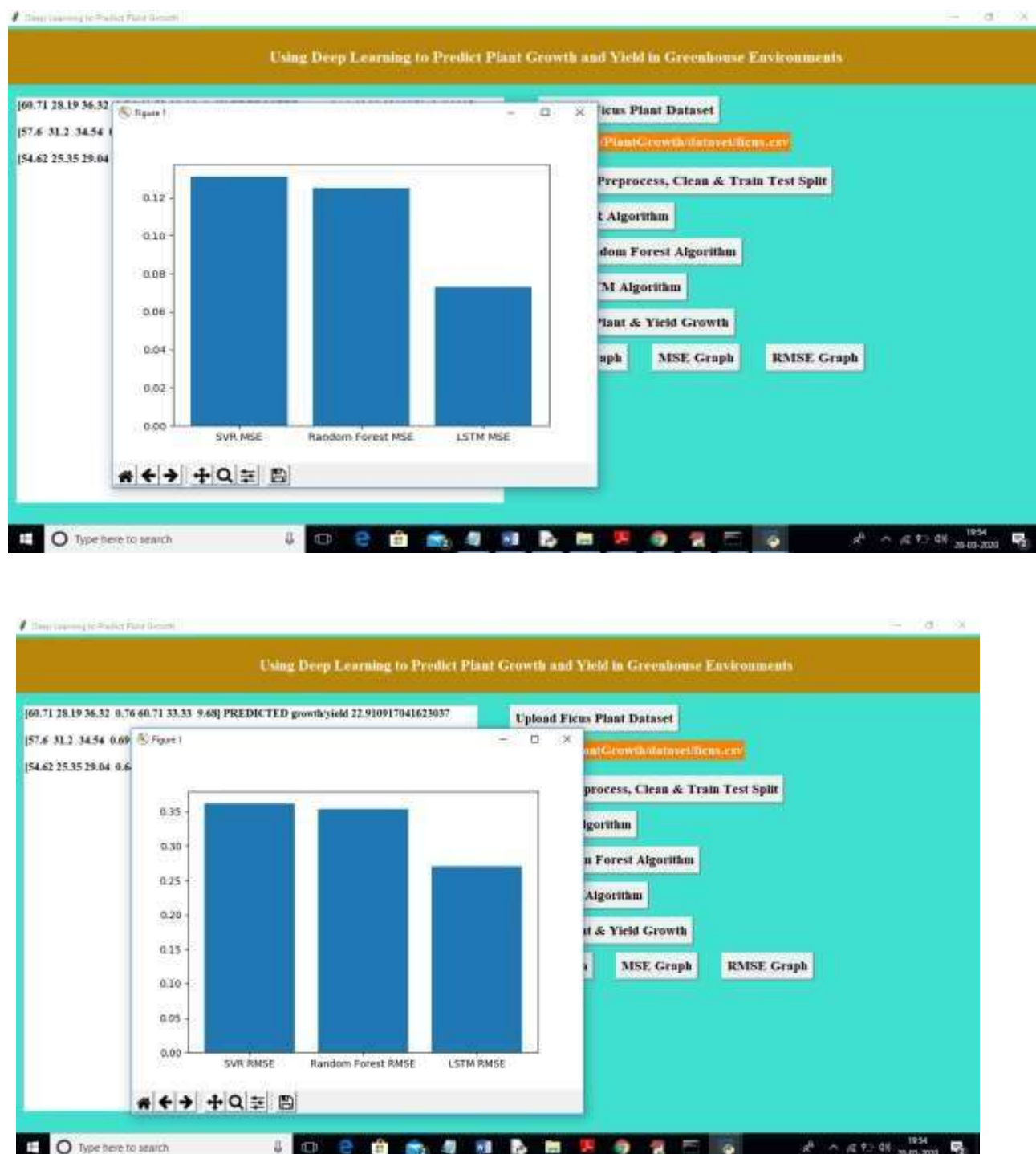
Fig8:RMSEgraph
