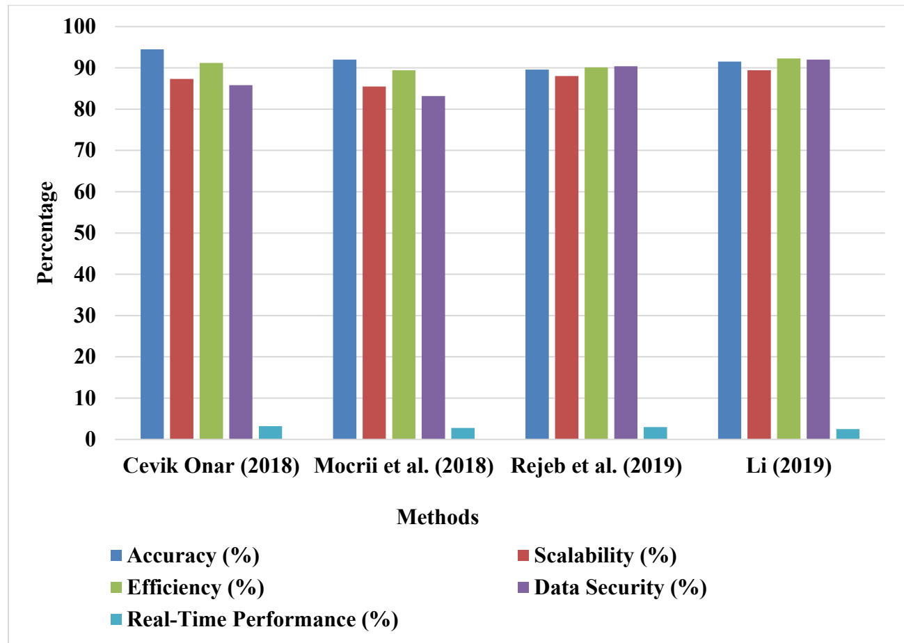
Figure 3 Performance Comparison of IoT and Healthcare Methods Across Key Metrics
