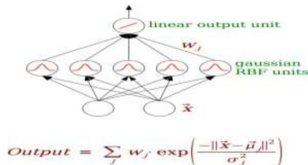
Fig -2: RBF Network
