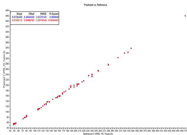
Fig.1. Partial Least Square of water property and sugarcane yield projection of the factors and instance.
