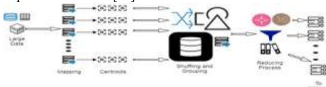
Fig.3.Map-Reducing Process[16]
