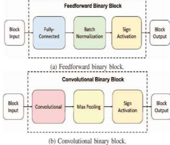
Fig. 1: Binary blocks
