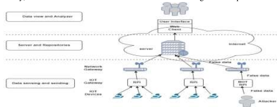
Figure 1: Botnet attack model
