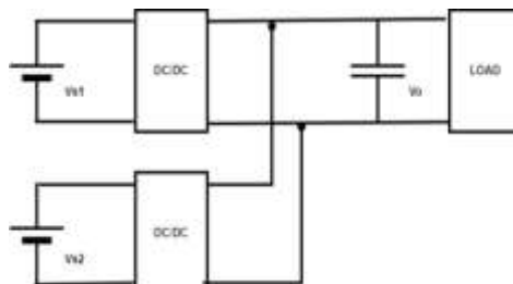
Fig.3. Common DC
