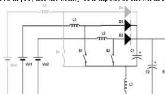
Fig. 5. n-input converter
