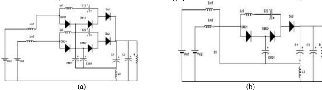
Fig. 7. Proposed Topology
