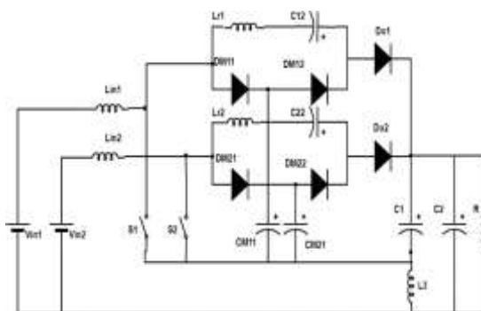
Fig. 7. Proposed Topology
