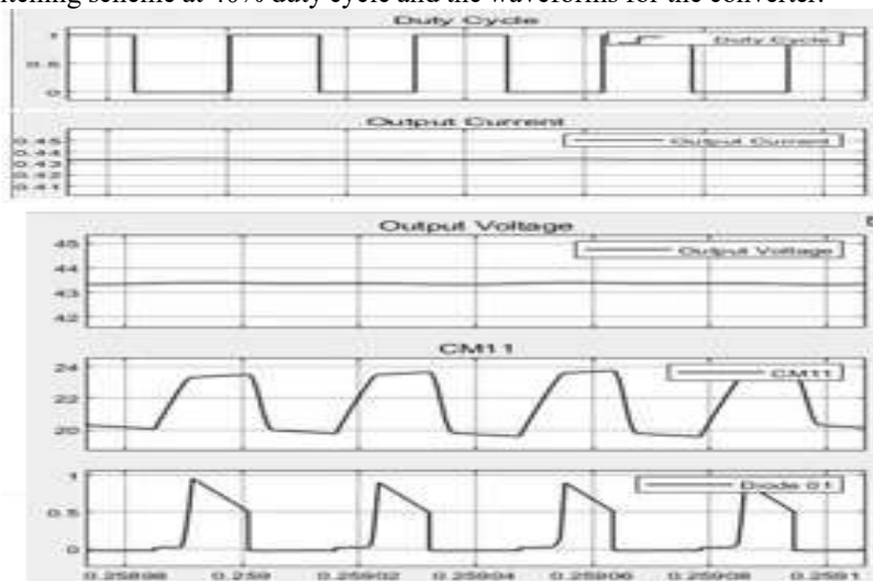
Fig. 9. Switching Scheme: Duty Cycle (40%), Output Current, Output Voltage, Capacitor Voltage CM11 and Diode Current Do1
