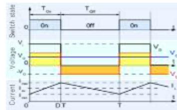
Fig. 4: Evolution of the voltages and currents with time in an ideal buck converter operating in continuous mode.
