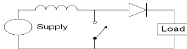
The basic schematic of a boost converter. The switch is typically a MOSFET, IGBT, or BJT.
