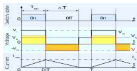
Fig. 5: Evolution of the voltages and currents with time in an ideal buck converter operating in discontinuous mode.
