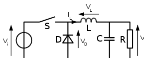
Fig. 3: Naming conventions of the components, voltages and current of the buck converter.
