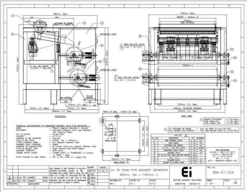
Fig.1: Line Diagram of Magnetic Separator.
