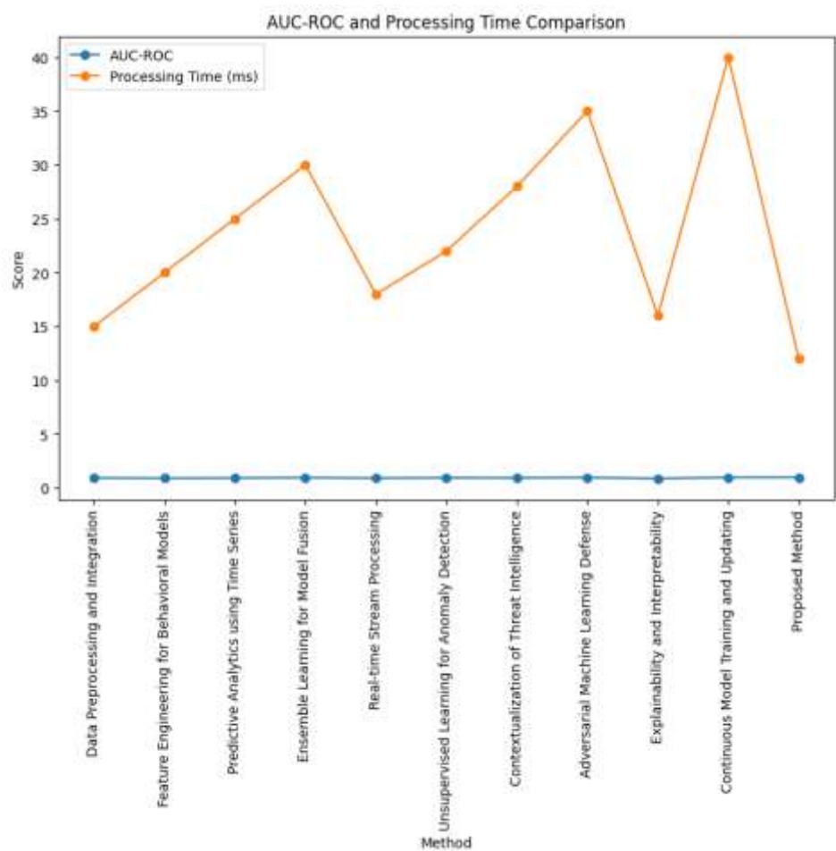
Figure.6.Comparative analysis of AUC-ROC and processing time for methods.
