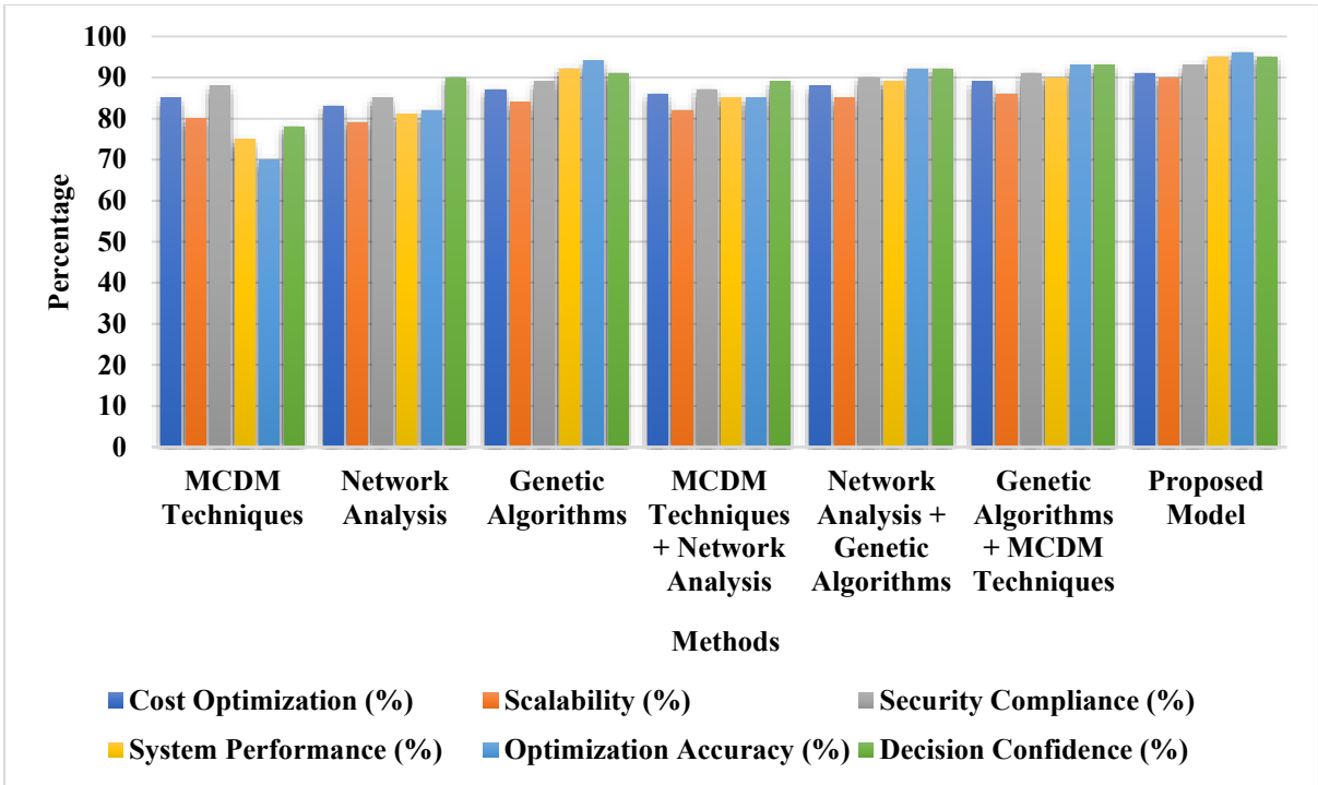
Figure 3 Ablation Study of MCDM, Network Analysis, and Genetic Algorithms Integration
