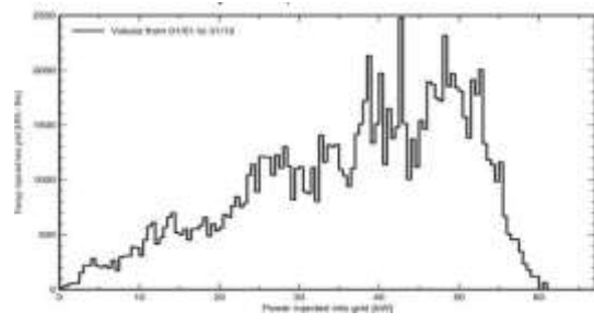
FIGURE 7. System output power distribution
