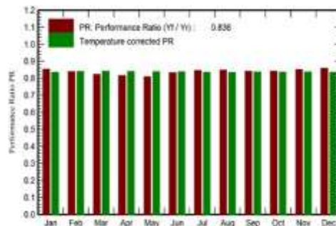
FIGURE 3. Performance ratio.
